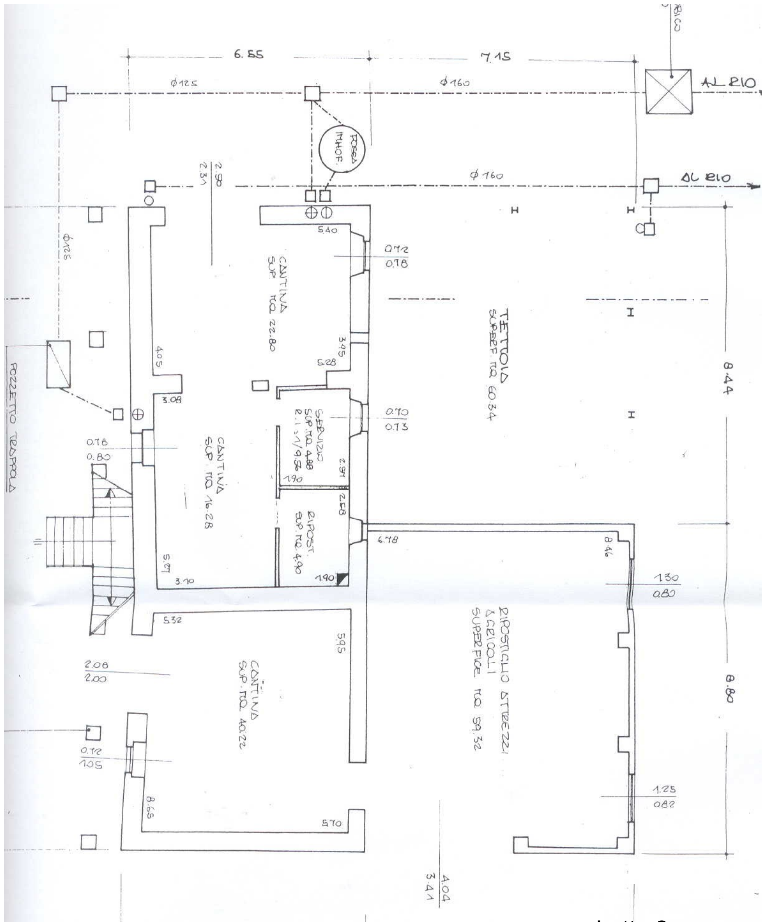
Lotto 2 Piano Terra
